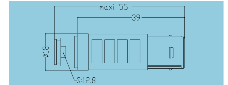
With cable collet and nut for fitting a bend relief
