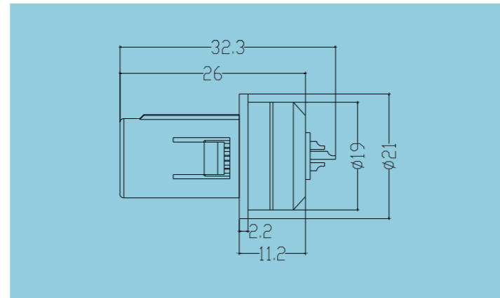
Short plug
